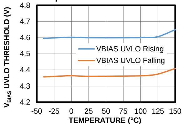
V_{BIAS} UVLO Threshold vs. Temperature
