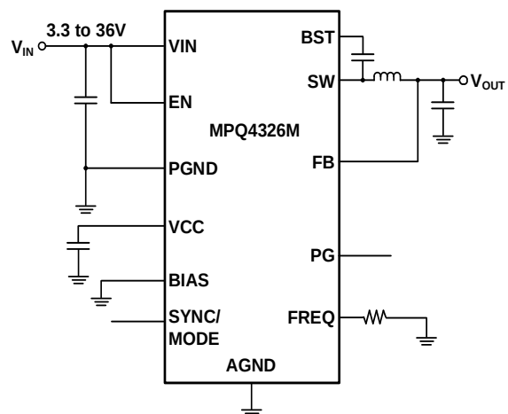
Fixed-Output Version
