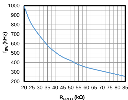
Figure 8: f_{SW} vs. R_{FREQ} (200kHz to 1000kHz)
