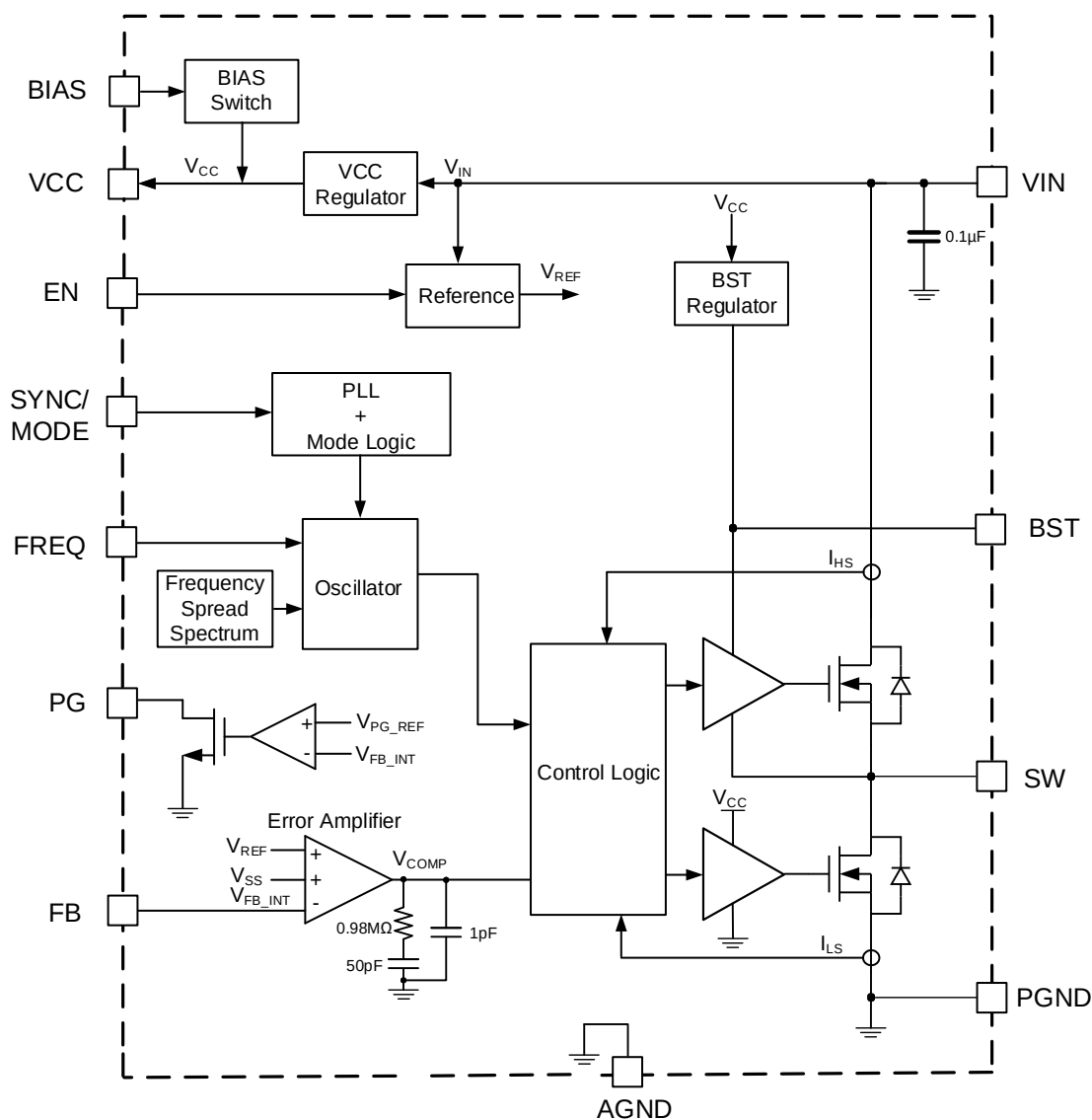
Figure 1: Adjustable-Output Version Functional Block Diagram
