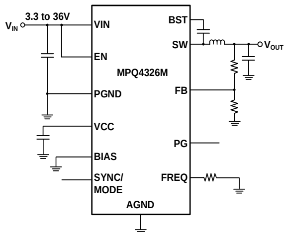
Adjustable-Output Version
