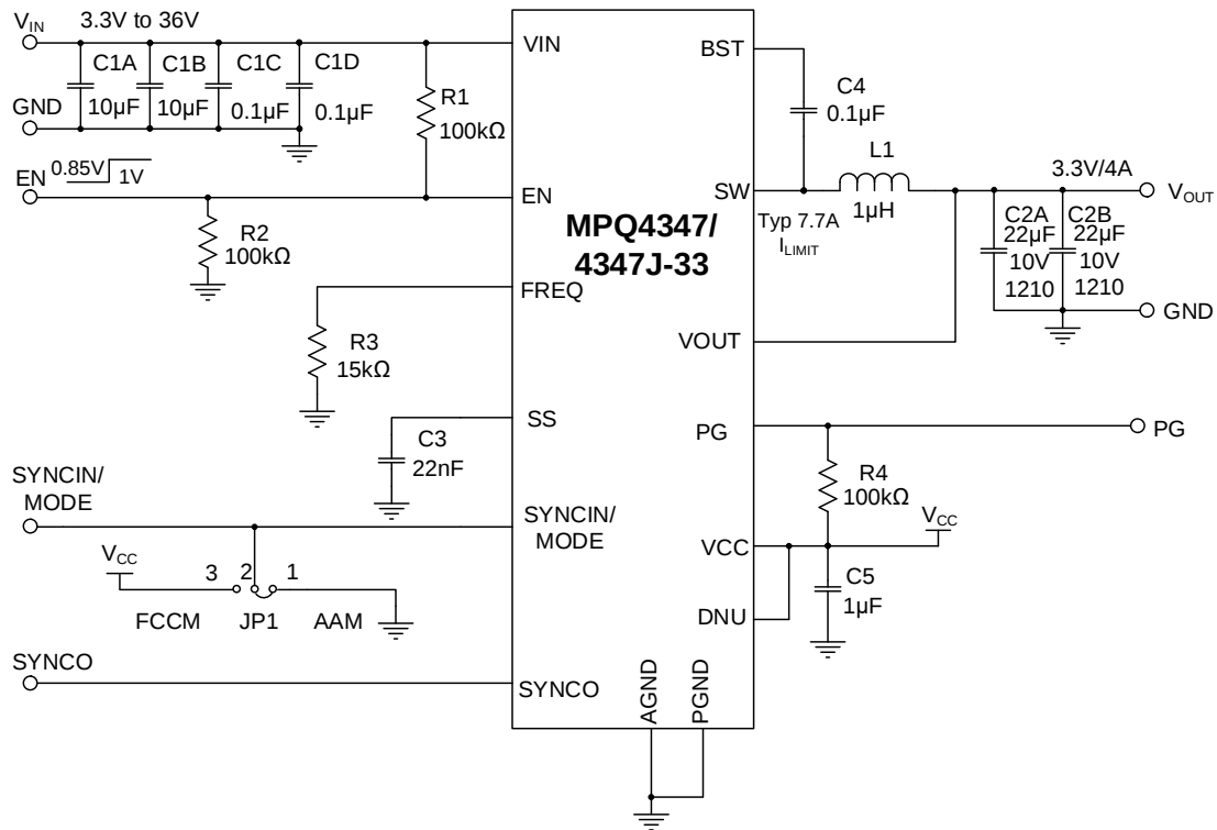
Figure 13: Typical Application Circuit ( V_{OUT} = 3.3\text{V} , f_{sw} = 2.2\text{MHz} )
