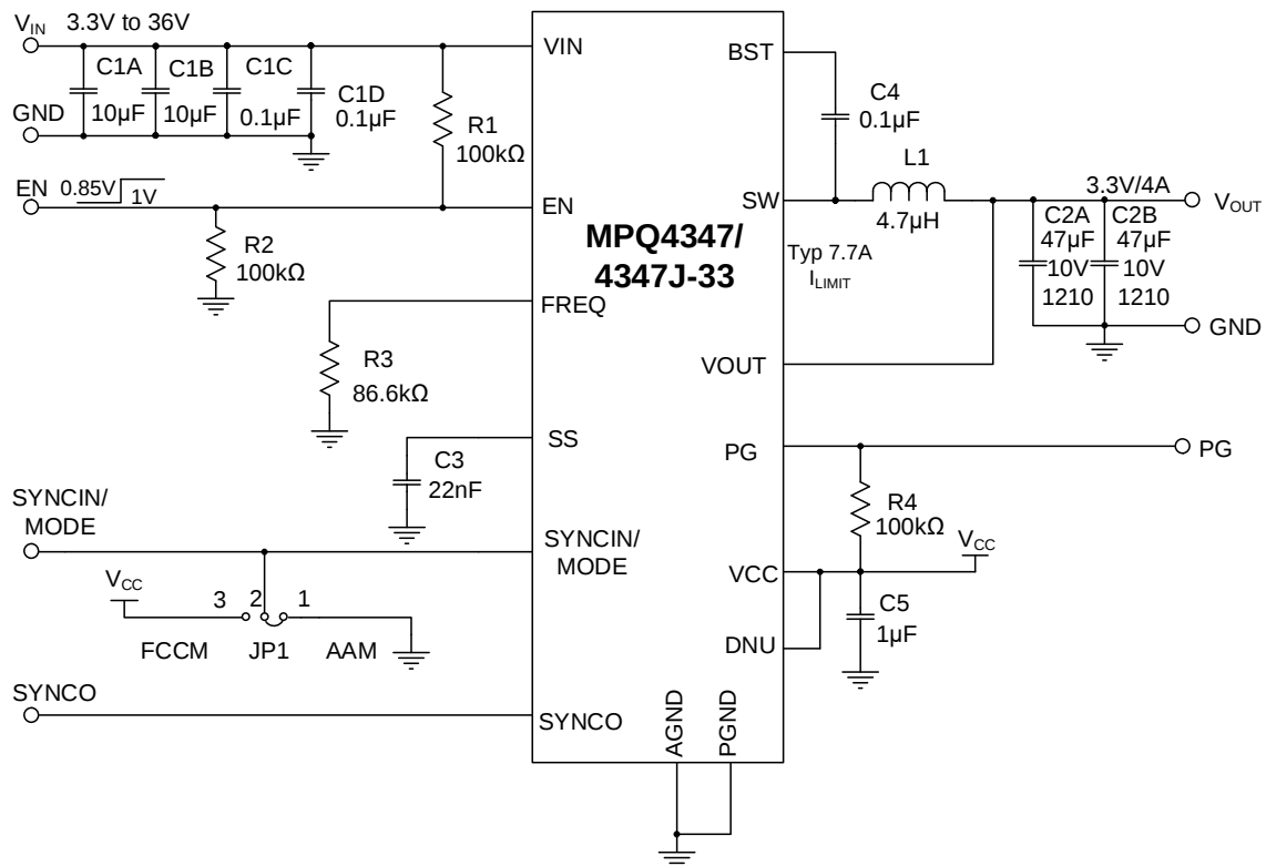
Figure 14: Typical Application Circuit ( V_{OUT} = 3.3\text{V} , f_{sw} = 410\text{kHz} )
