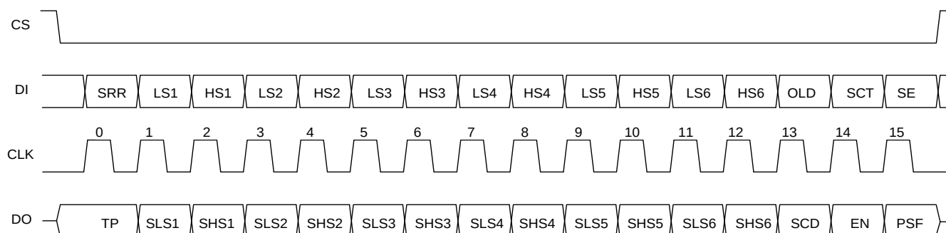
Figure 2: Data Transfer
