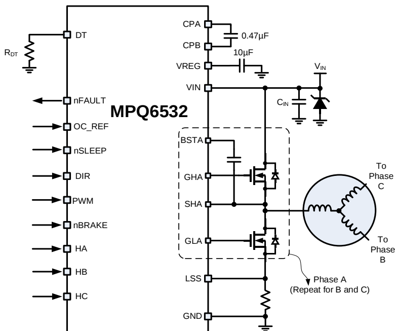
Figure 8: Typical Application Circuit
