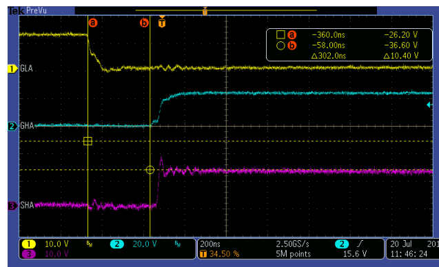
Figure 2: Dead Time
