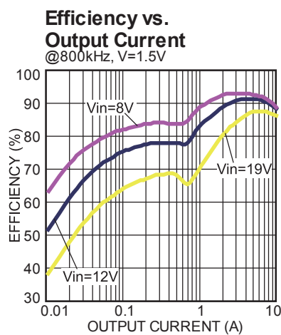
Figure 36 — Efficiency Curve
