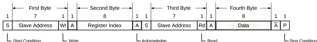
Figure 25: Read Sequence (9)
