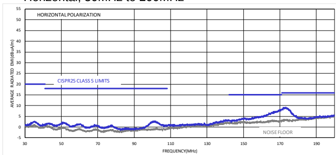
CISPR25 Class 5 Average Radiated Emissions Horizontal, 30MHz to 200MHz
