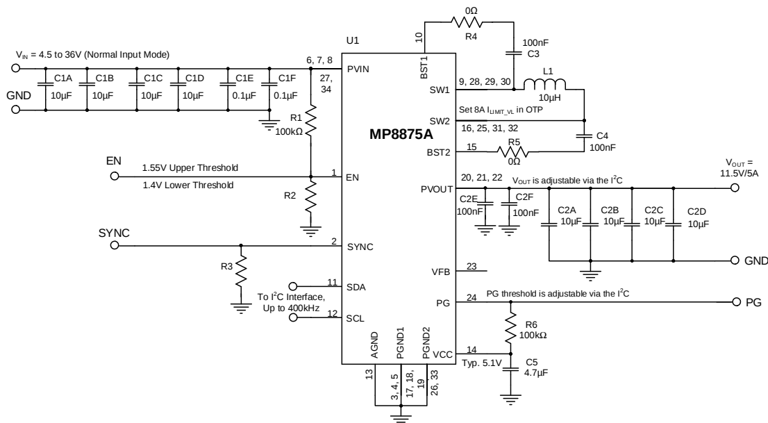
Figure 28: Typical Application Circuit, V OUT = 11.5V, f sw = 450kHz
