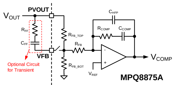
Figure 15: Compensation Network
