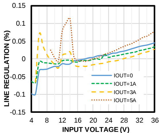
Line Regulation
