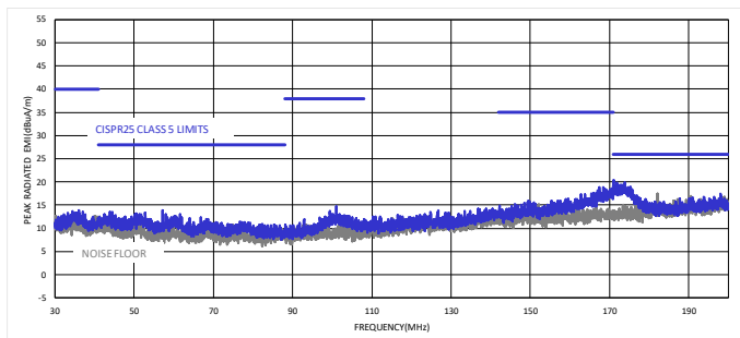
CISPR25 Class 5 Peak Radiated Emissions Horizontal, 30MHz to 200MHz
