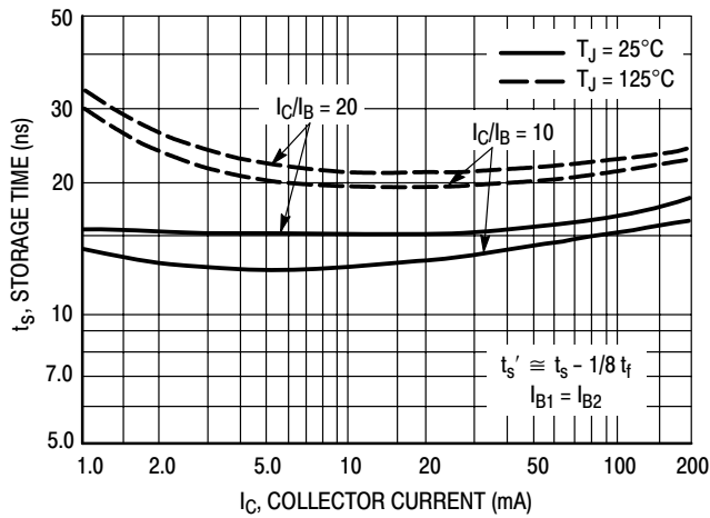
Figure 9. Storage Time
