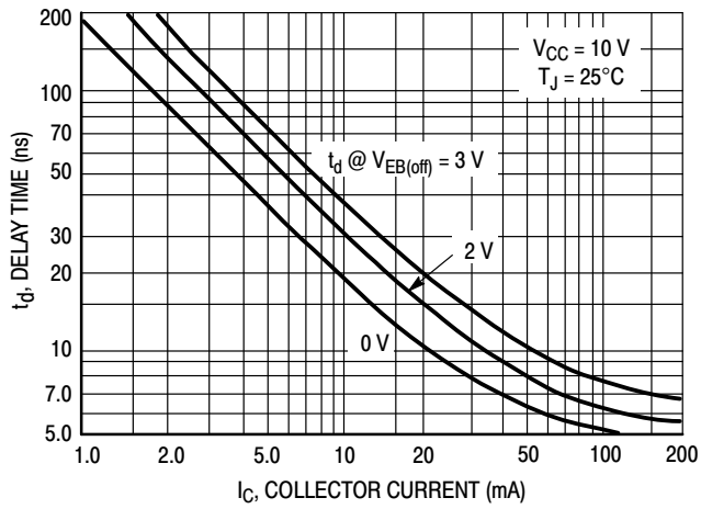
Figure 7. Delay Time
