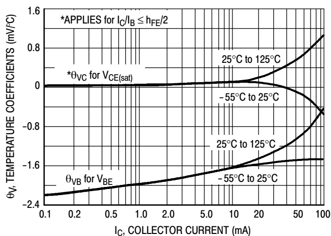
Figure 5. Temperature Coefficients
