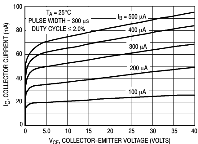
Figure 3. Collector Characteristics
