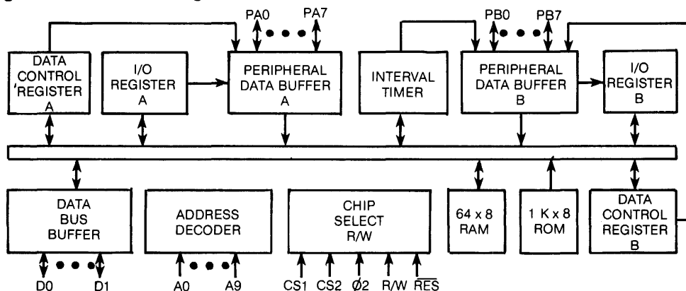
Figure 1. 6530 Block Diagram
