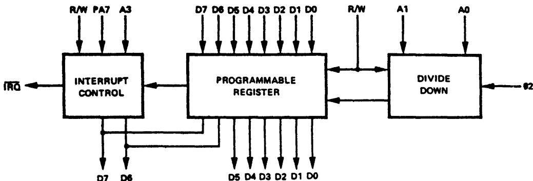
Figure 2. BASIC ELEMENTS OF INTERVAL TIMER
