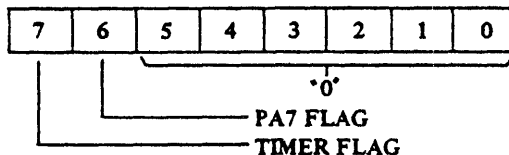
Figure 4. INTERRUPT FLAG REGISTER
