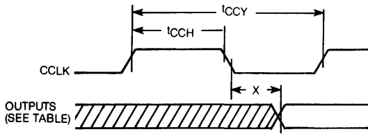
SYSTEM TIMING
