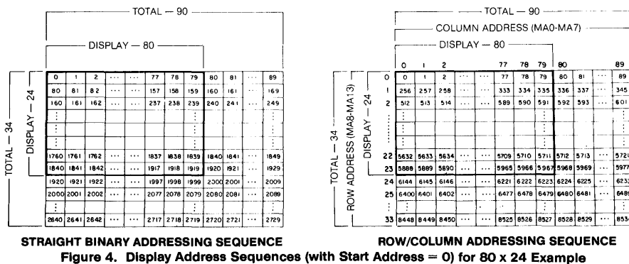
Figure 4. Display Address Sequences (with Start Address = 0) for 80 x 24 Example
