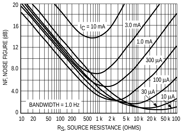
Figure 7. Noise Figure
