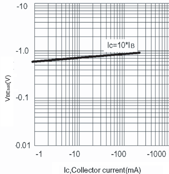
FIG3. BASE-EMITTER
