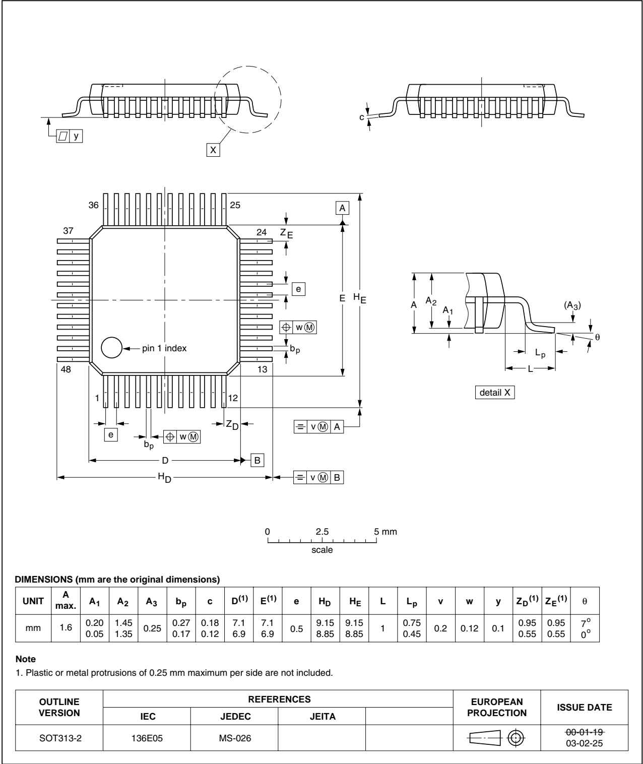
Fig 6. Package outline
