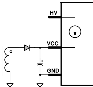
Figure 13: Start-Up Circuit
