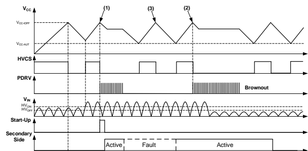
Figure 2: Start-Up Logic for the Primary IC
