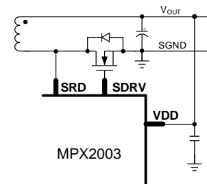
Figure 8: V_{DD} Supply from the Output
