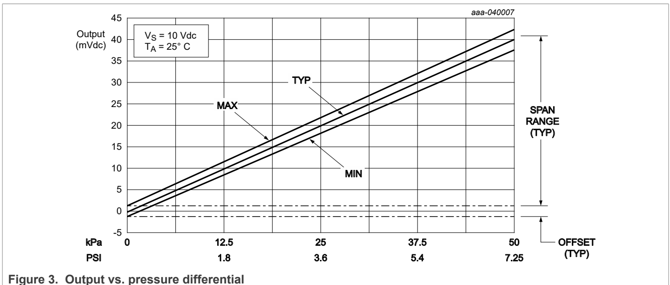
Figure 3. Output vs. pressure differential
