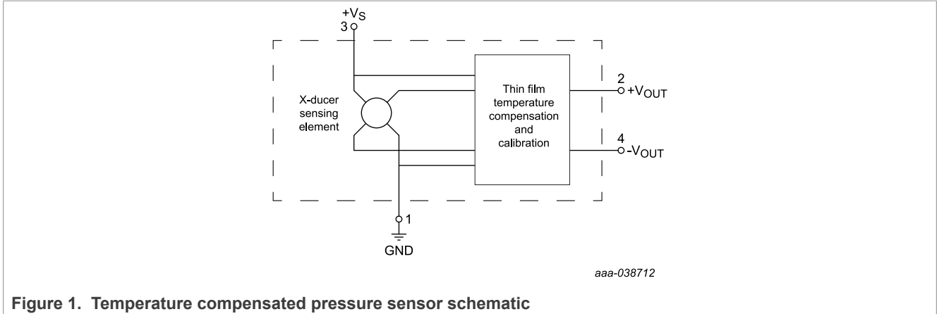
Figure 1. Temperature compensated pressure sensor schematic
