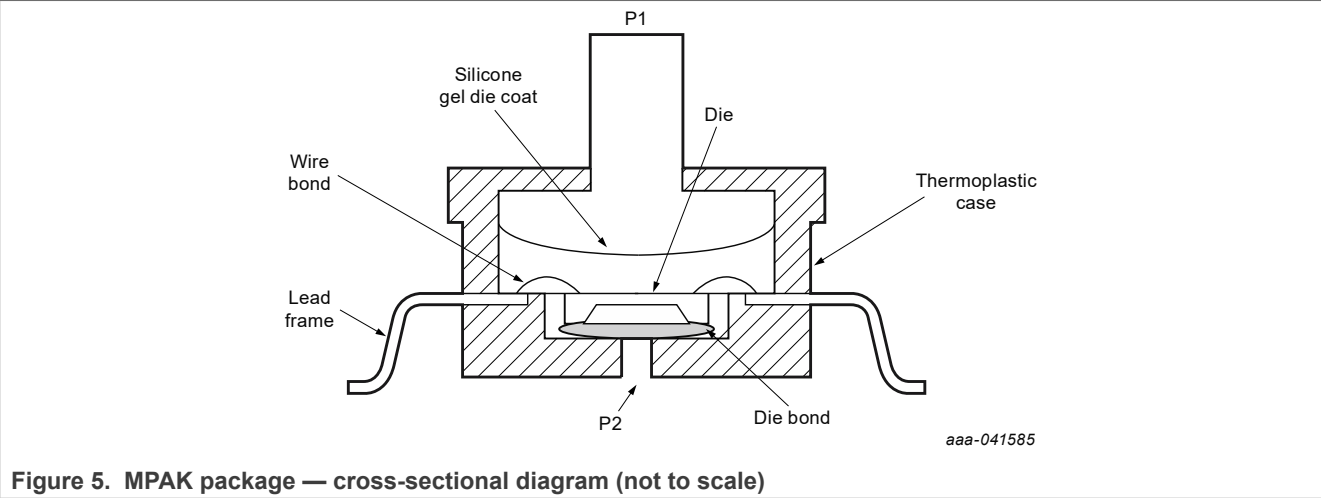
Figure 5. MPAK package — cross-sectional diagram (not to scale)
