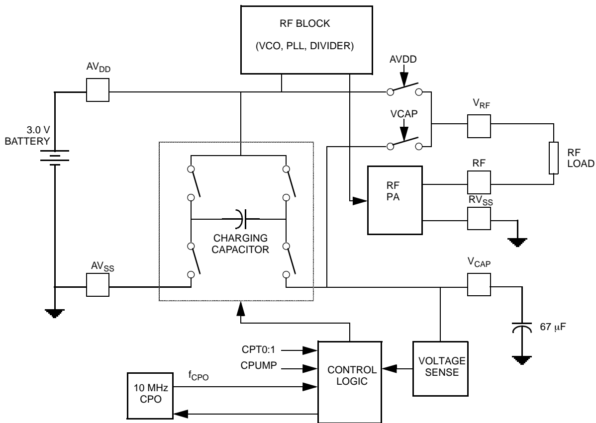
Figure 13-16 RFX Charge Pump Block Diagram
