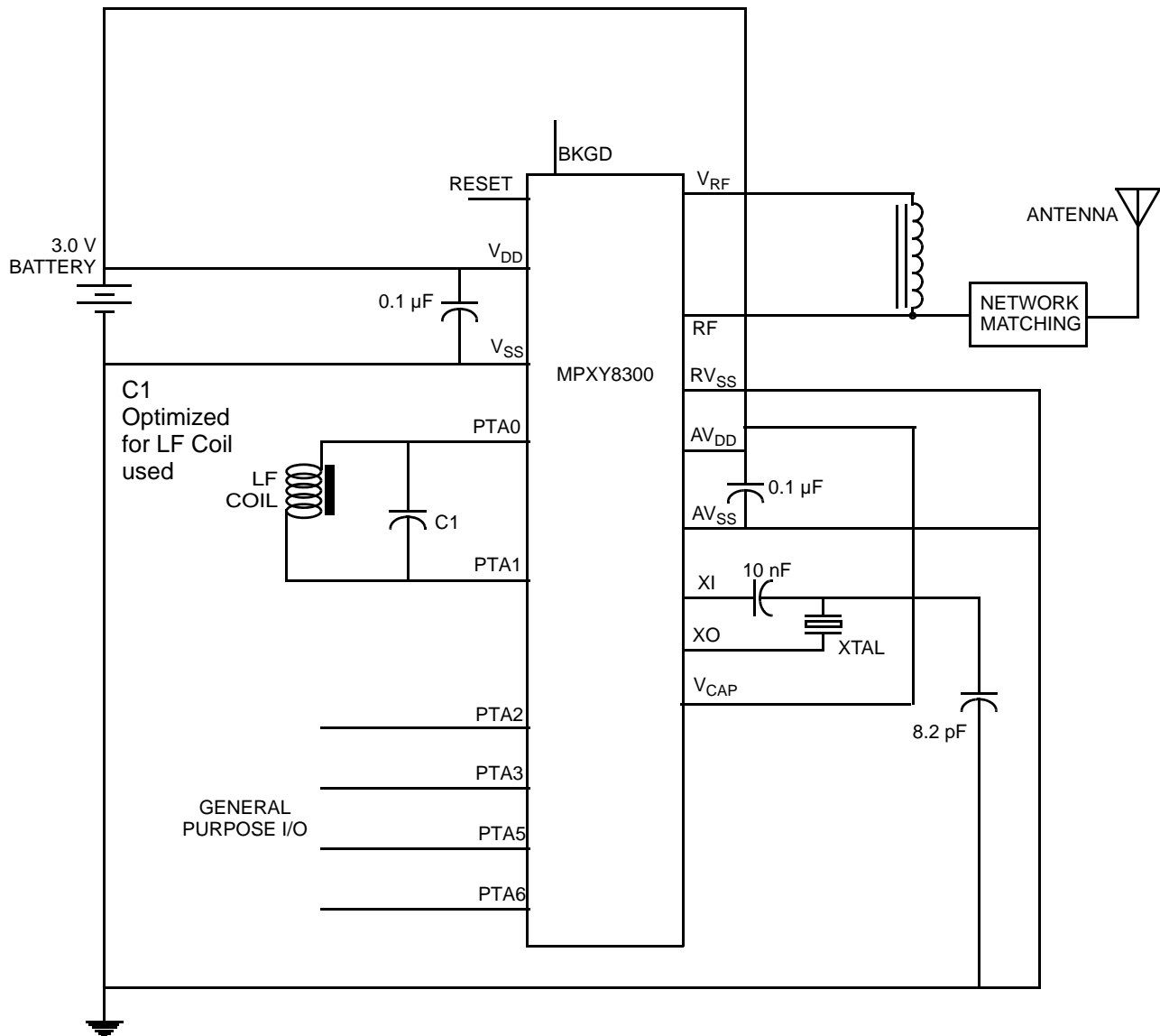
Figure 2-3 MPXY8300 Series Example Application
