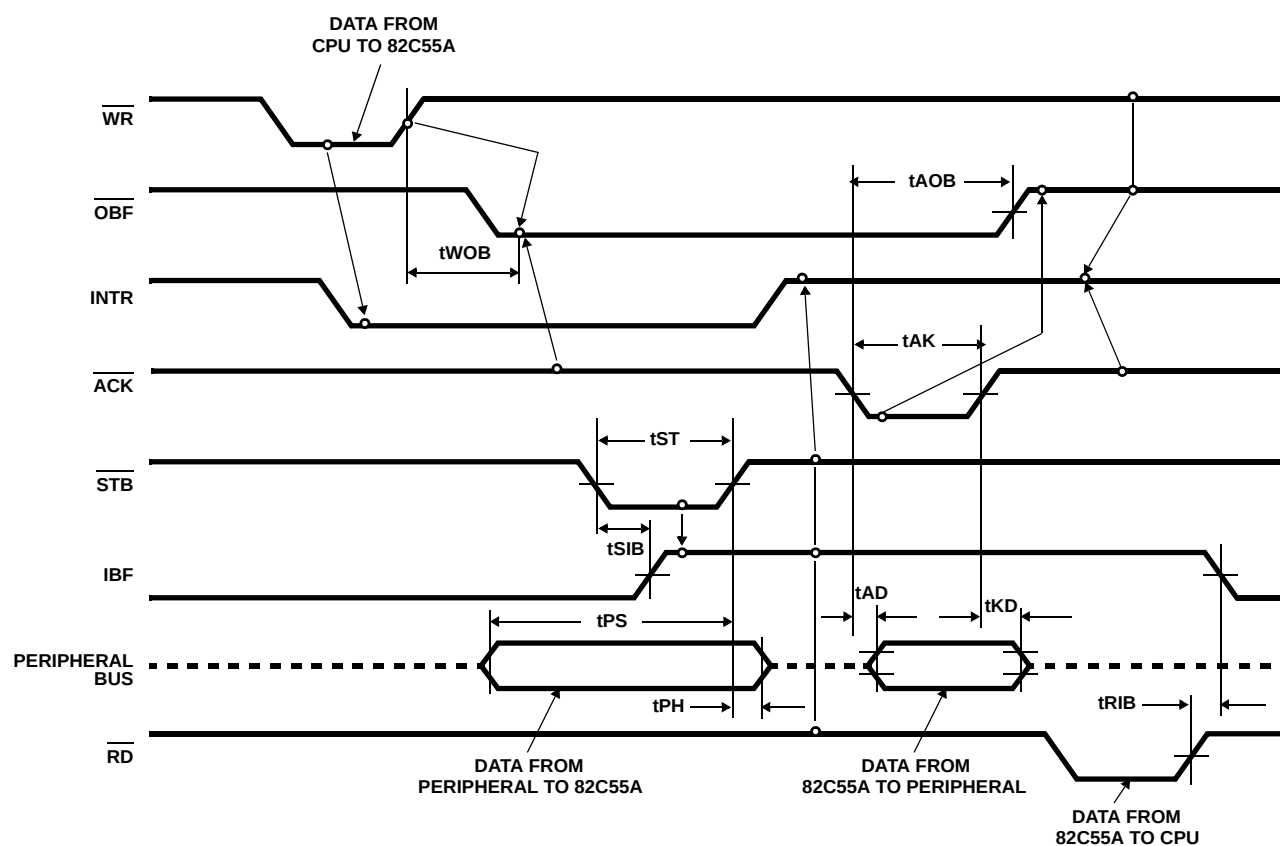
FIGURE 13. MODE 2 (BIDIRECTIONAL)
