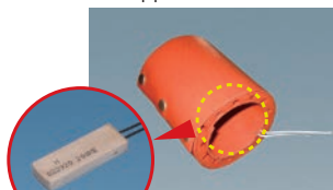
MQT8H 3XC Freeze protection of residential water pipe
