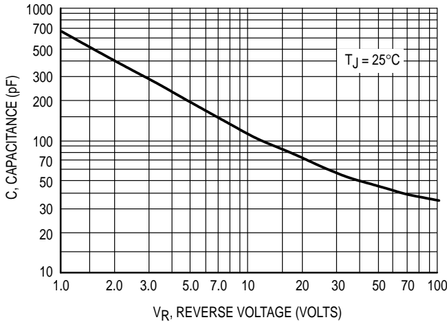
Figure 11. Junction Capacitance
