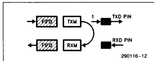
Figure 13. Local Loopback
