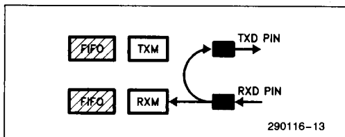
Figure 14. Remote Loopback
