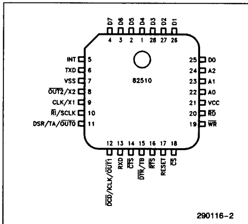
Figure 2. PLCC Pinout
