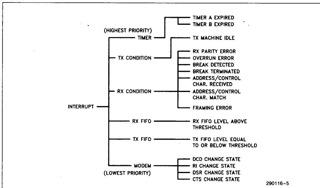
Figure 5. Interrupt Structure
