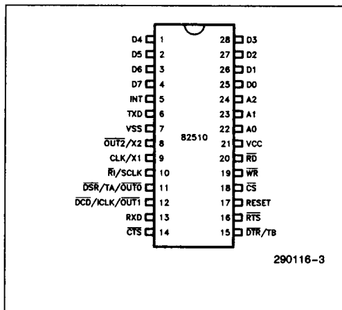
Figure 3. DIP Pinout
