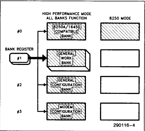
Figure 4. 82510 Register Architecture
