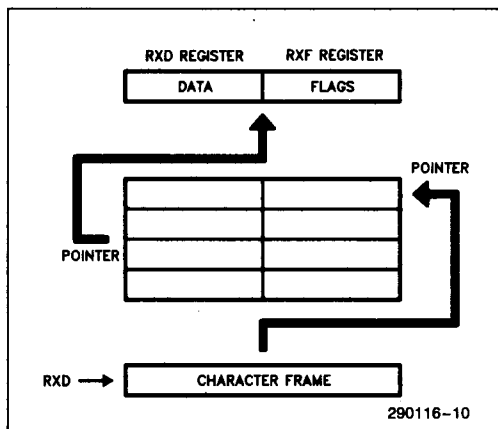
Figure 10. Rx FIFO
