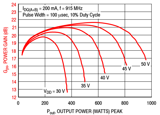
Figure 18. Power Gain versus Output Power and Drain-Source Voltage
