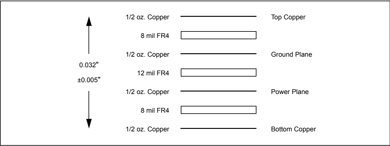
FIGURE 2-9: PCB LAYER STACK UP
