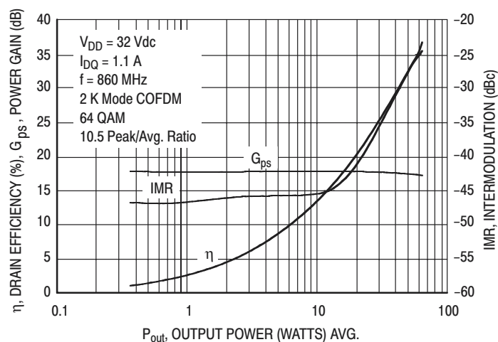
Figure 8. COFDM Intermodulation, Gain and Efficiency versus Output Power in Broadband Circuit
