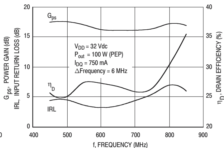
Figure 6. Performance in Broadband Circuit
