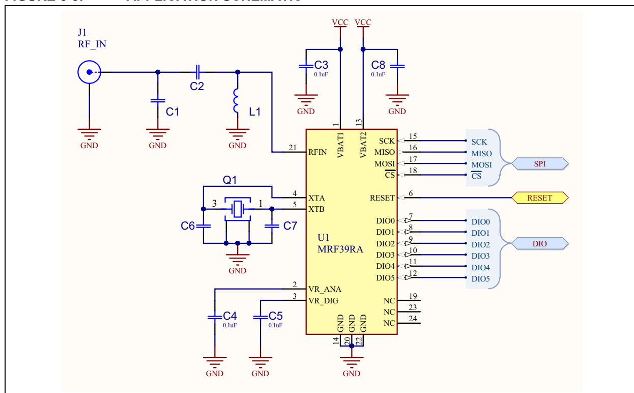
FIGURE 6-3: APPLICATION SCHEMATIC
