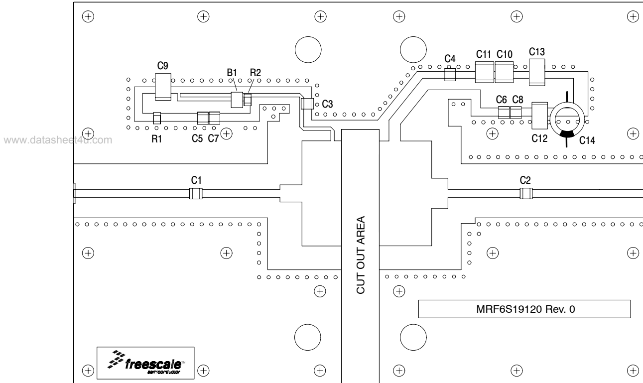
Figure 2. MRF6S19120HR3(SR3) Test Circuit Component Layout
