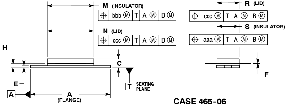
CASE 465-06 ISSUE G NI-780 MRF6S19120HR3
