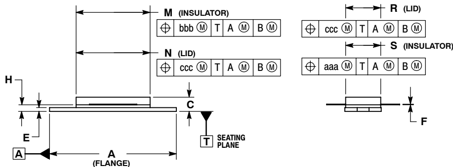
CASE 465-06 ISSUE G NI-780 MRF6S19200HR3
