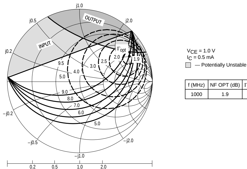
Figure 18. Constant Gain and Noise Figure Contours
