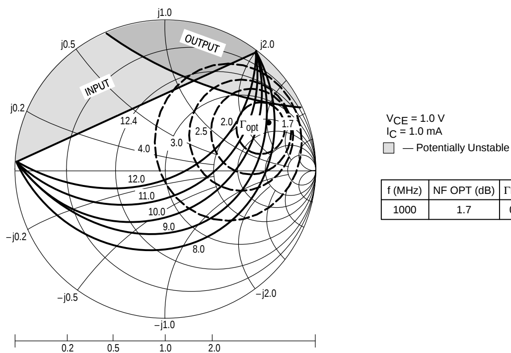
Figure 19. Constant Gain and Noise Figure Contours
