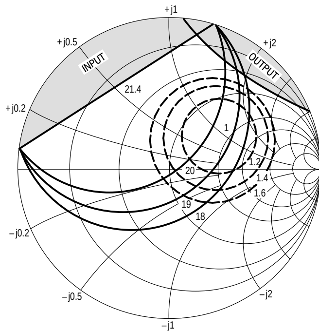
Figure 15. MRF941 Constant Gain and Noise Figure Contours (f = 0.5 GHz)
