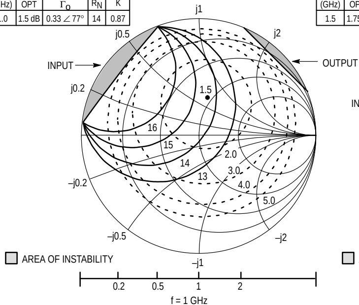
Figure 25. MRF947 Series Constant Gain and Noise Figure Contours
