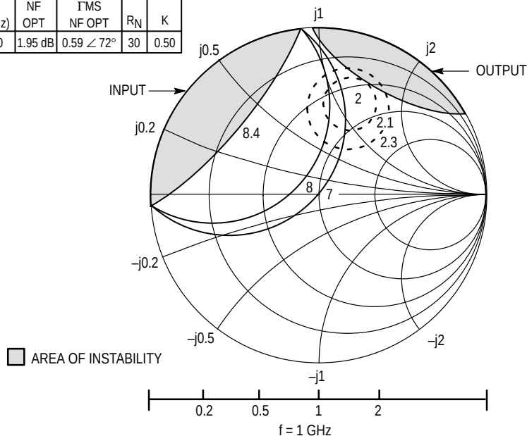
Figure 27. MRF947 Series Constant Gain and Noise Figure Contours
