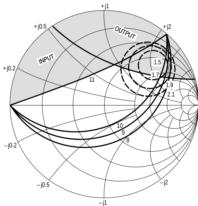
Figure 17. MMBR941LT1, T3 Constant Gain and Noise Figure Contours (f = 1.0 GHz)
