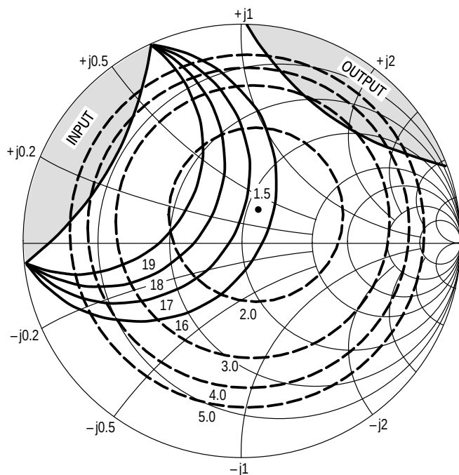
Figure 24. MRF9411LT1 Constant Gain and Noise Figure Contours (f = 1.0 GHz)
