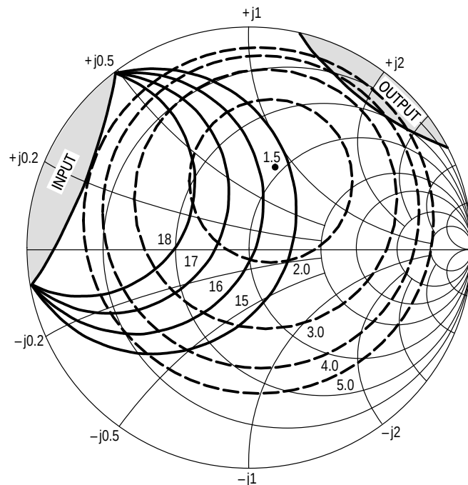
Figure 16. MRF941 Constant Gain and Noise Figure Contours (f = 1.0 GHz)
