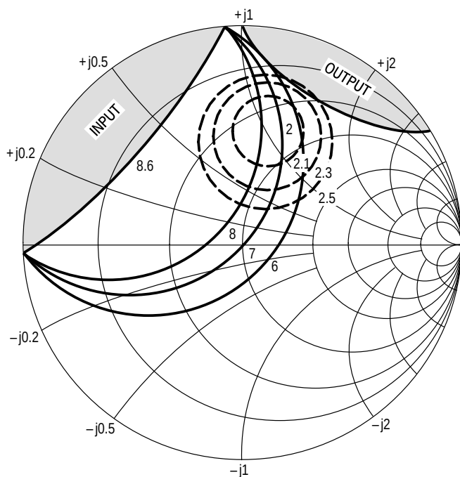
Figure 18. MMBR941LT1, T3 Constant Gain and Noise Figure Contours (f = 0.5 GHz)
