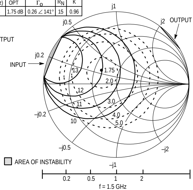
Figure 26. MRF947 Series Constant Gain and Noise Figure Contours
