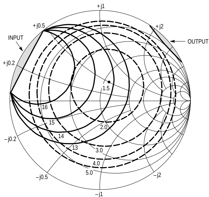
Figure 20. MMBR941LT1, T3 Constant Gain and Noise Figure Contours (f = 1.0 GHz)
