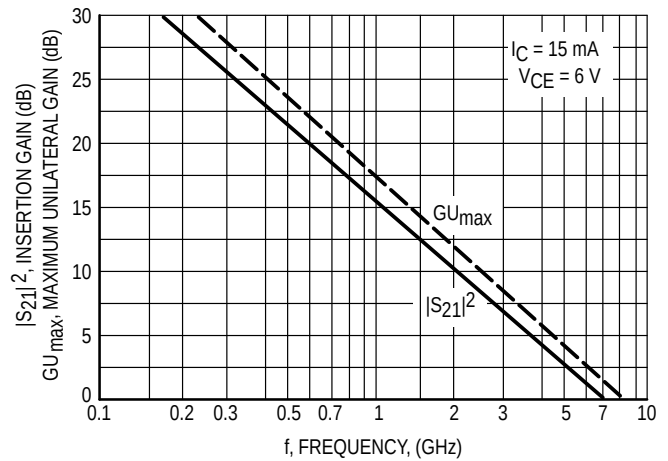
Figure 6. MRF941, MRF9411LT1
