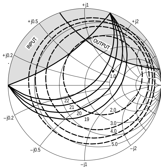
Figure 23. MRF9411LT1 Constant Gain and Noise Figure Contours (f = 0.5 GHz)
