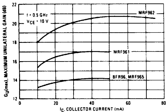
FIGURE 3 – MAXIMUM UNILATERAL GAIN versus COLLECTOR CURRENT
