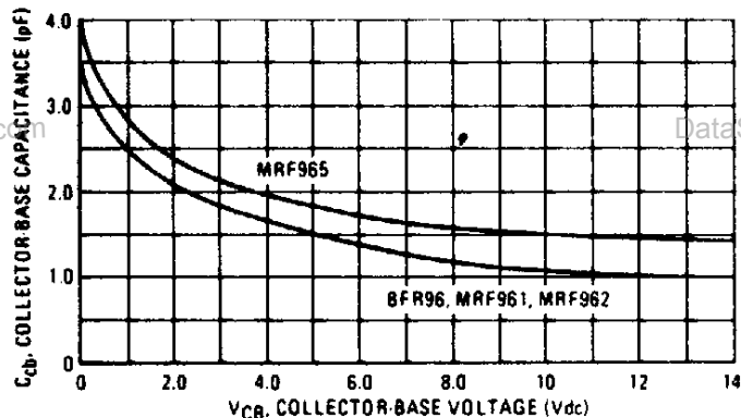
FIGURE 7 – COLLECTOR-BASE CAPACITANCE versus COLLECTOR-BASE VOLTAGE
