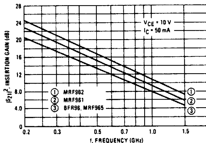
FIGURE 2 – |S_{21}|^2 versus FREQUENCY
