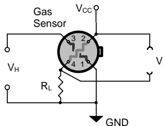
Figure 3: Measurement circuit for O 3 detection.
