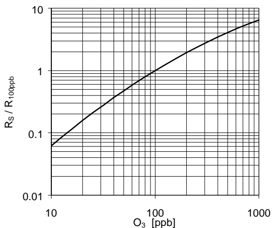
Figure 1: R_S / R_{100\text{ppb}} as a function of gas concentration at 50% RH and 25°C.
