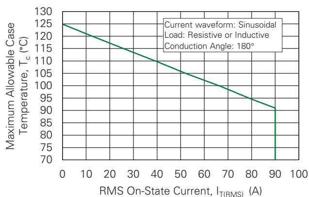
Fig. 6. Maximum Allowable Case Temperature vs. RMS On-state Current (per module)
