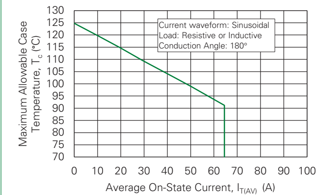
Fig. 7. Maximum Allowable Case Temperature vs. Average On-state Current (per module)
