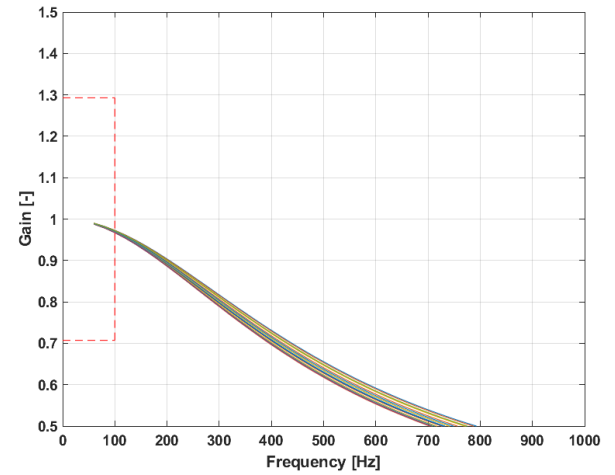
Figure 10 : Frequency response
