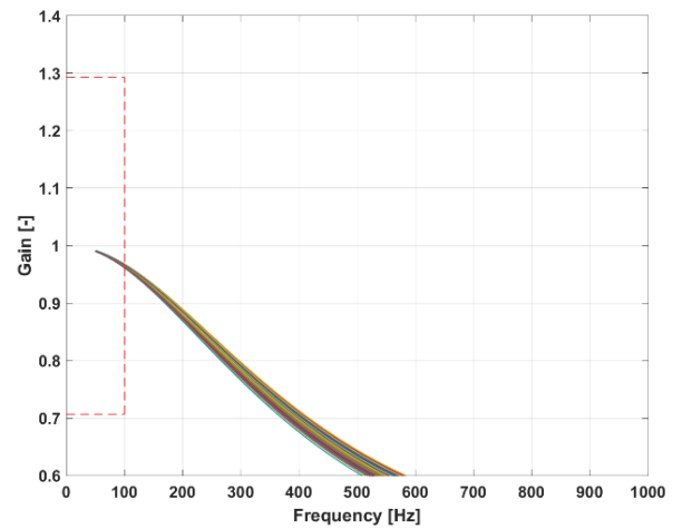
Figure 28 : Frequency response
