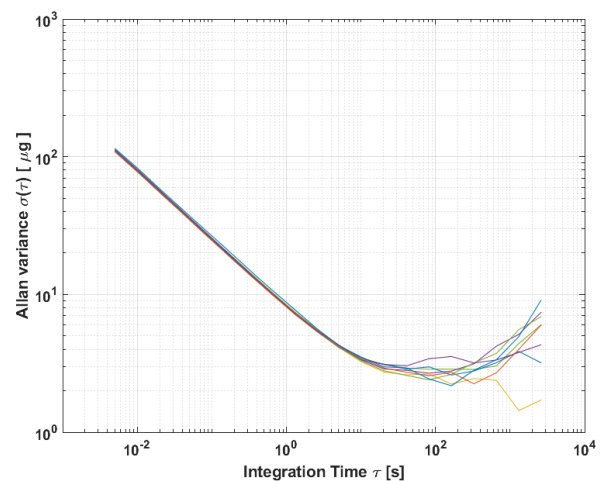
Figure 12: Allan Variance
