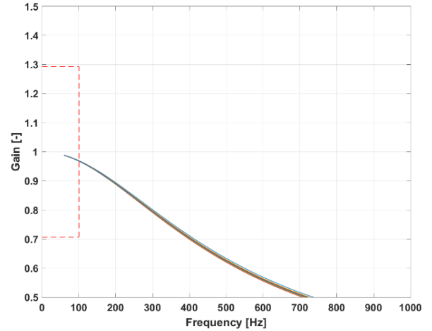
Figure 34 : Frequency response
