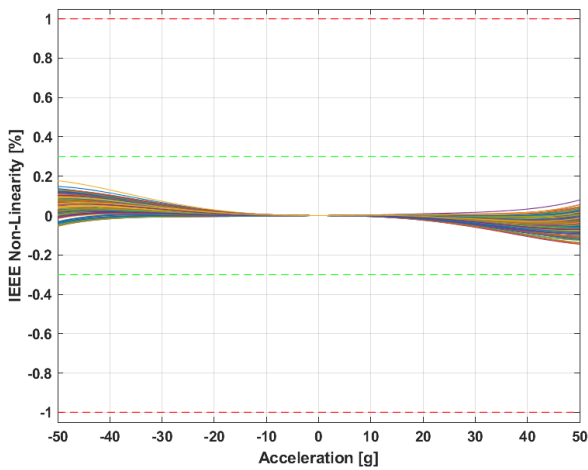
Figure 27 : Non-linearity IEEE
