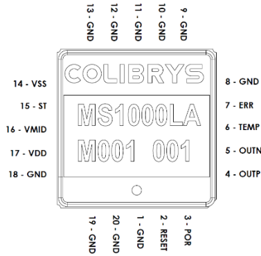
Figure 37 : Pinout top view
