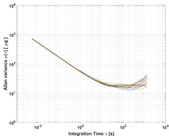
Figure 24: Allan Variance
