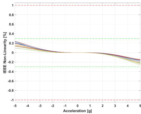
Figure 9 : Non-linearity IEEE
