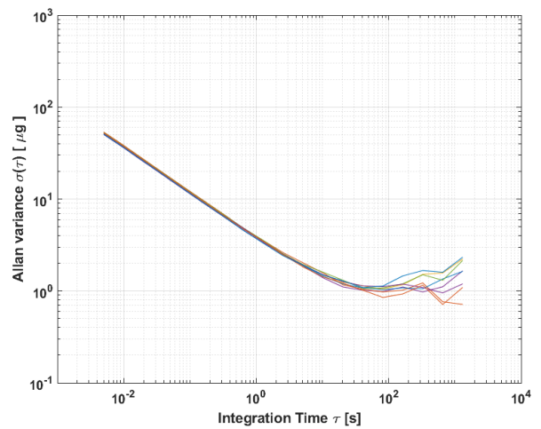
Figure 6: Allan Variance
