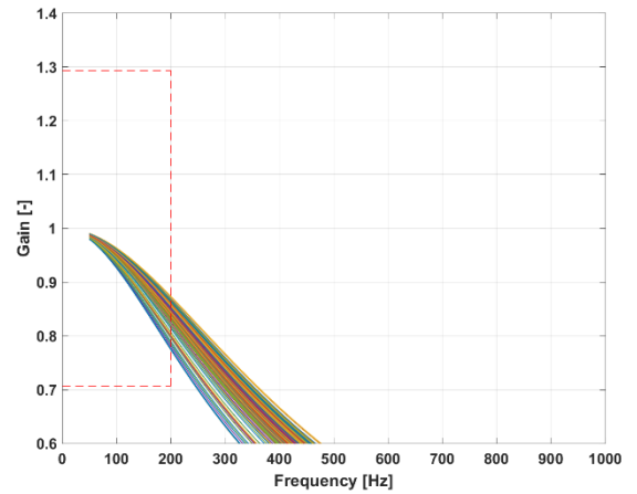
Figure 10 : Frequency response
