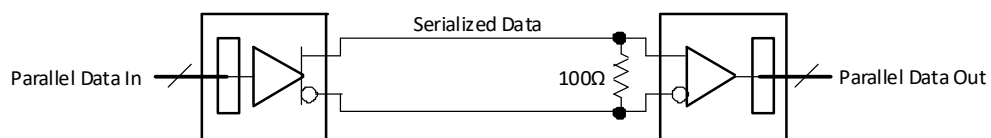
Figure 22. Single-ended Point-to-point Connection
