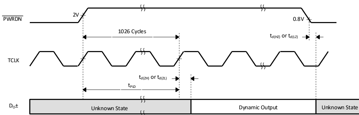
Figure 12. Serializer PLL Lock Time and PWRDN High-impedance-state Delay
