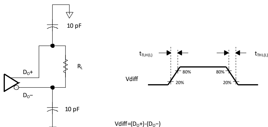
Figure 9. Serializer LVDS Output Load and Transition Time
