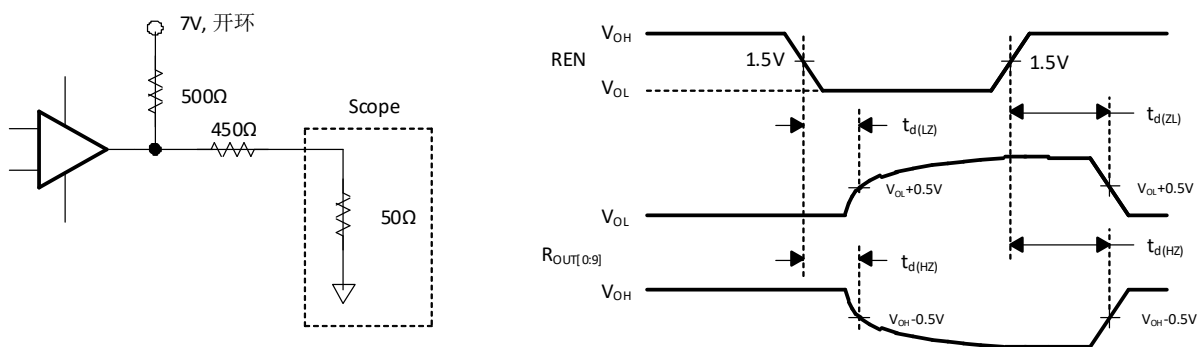
Figure 18. Deserializer High-impedance-state Test Circuit and Timing
