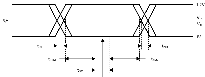
Figure 8. LVDS Input Margin Sampling
