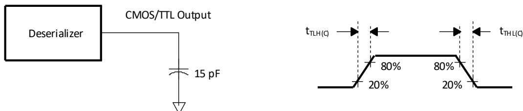
Figure 15. Deserializer CMOS/TTL Output Load and Transmission Time
