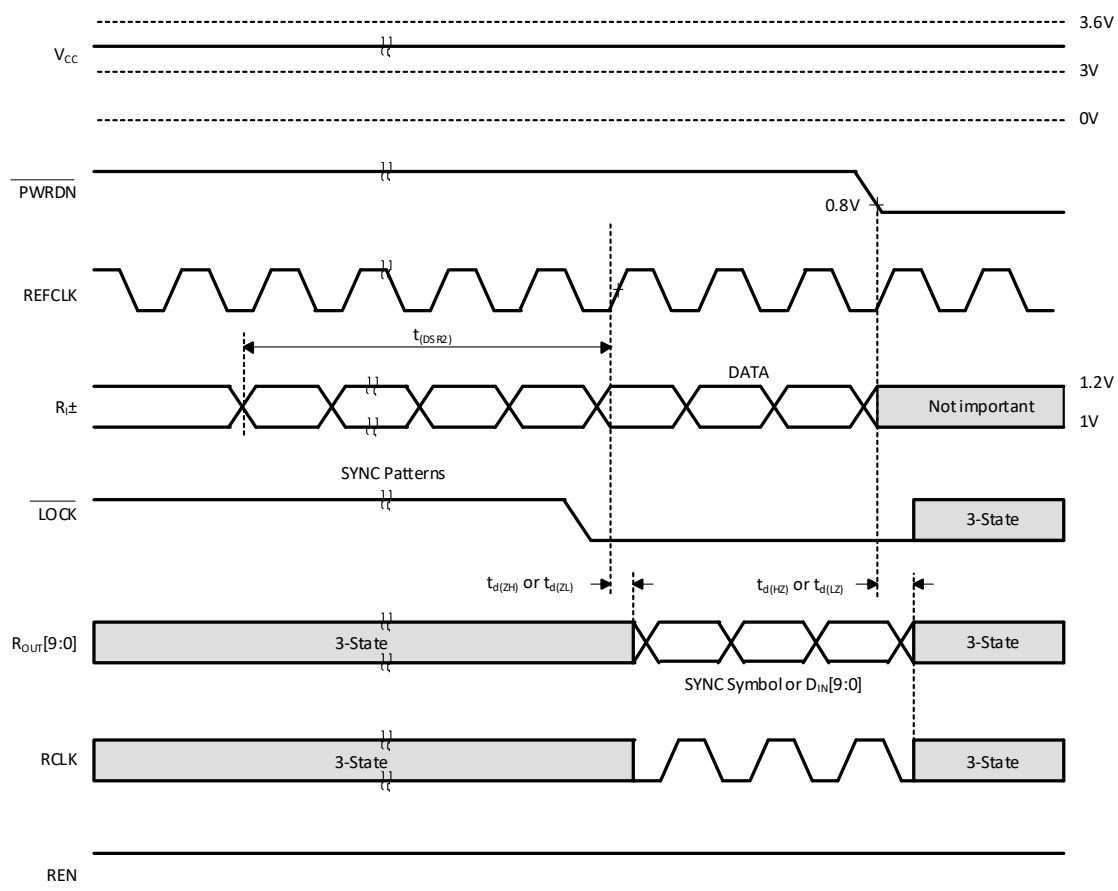
Figure 20. Deserializer PLL Lock Time during Synchronization
