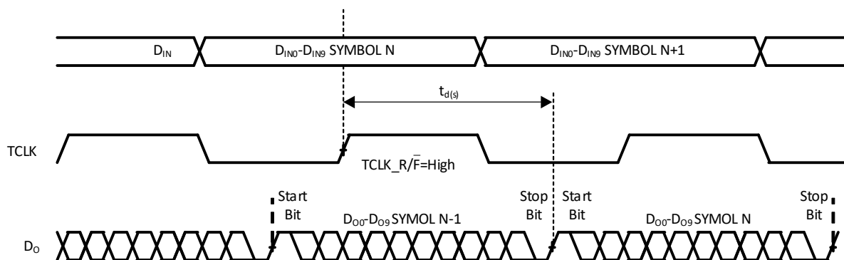
Figure 14. Serializer Delay
