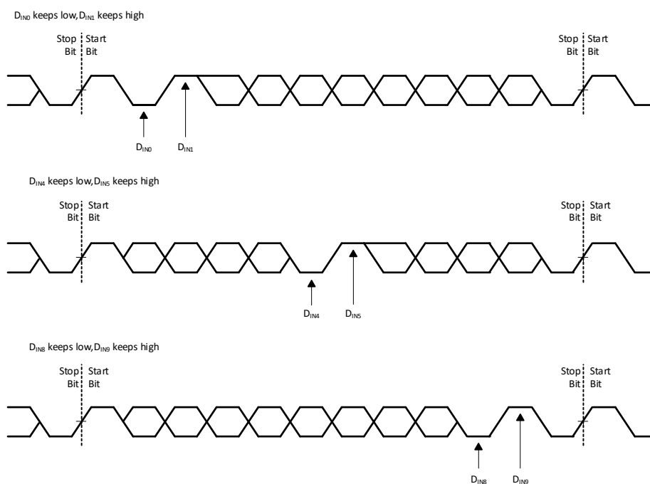
Figure 21. RMT Mode Example
