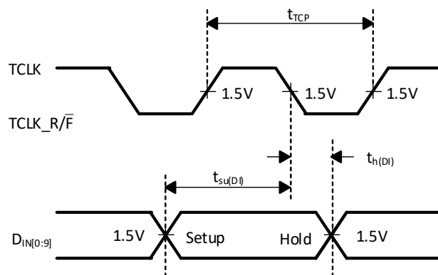
Figure 10. Serializer Setup/Hold Time
