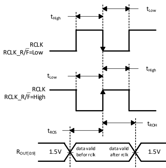
Figure 17. Deserializer Data Valid Output Timing
