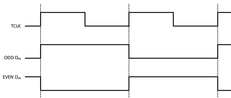
Figure 3. Worst-case Serializer I_{CC} Test Mode
