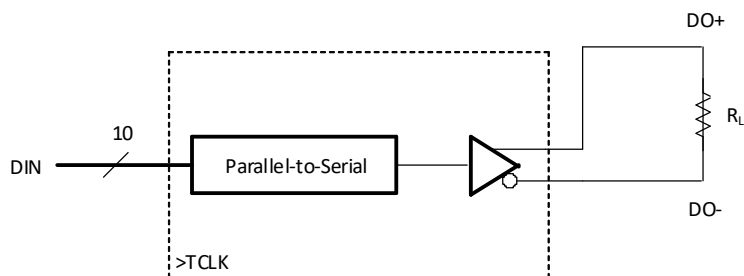
Figure 2. V_{OD} Output Diagram
