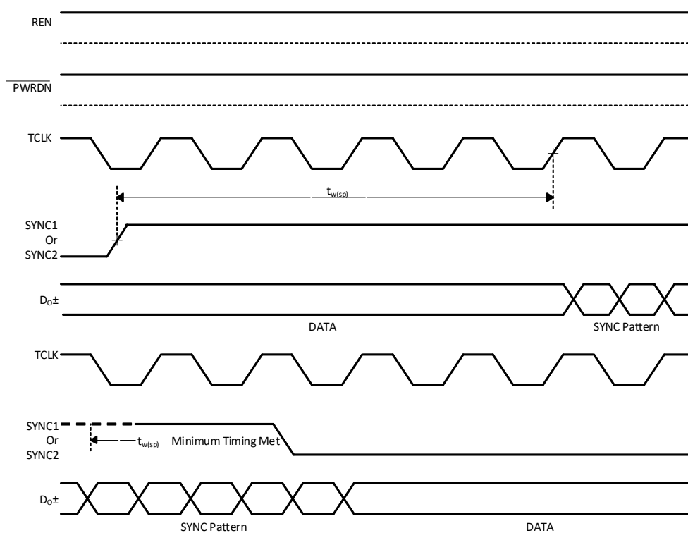
Figure 13. SYNC Timing Delay
