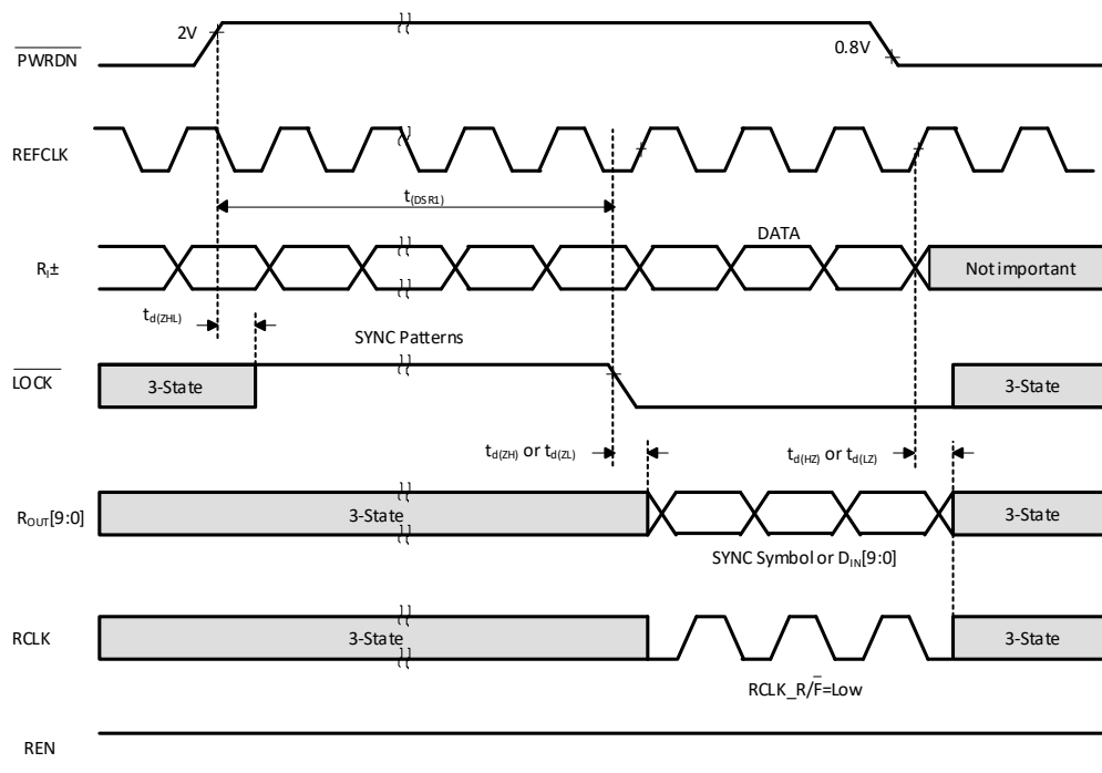
Figure 19. Deserializer PLL Lock Time and PWRDN 3-state Delay
