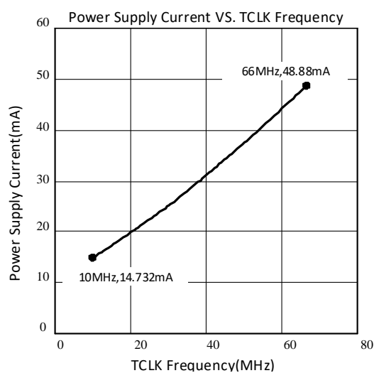
Figure 4. Power Supply Current VS. TCLK Frequency
