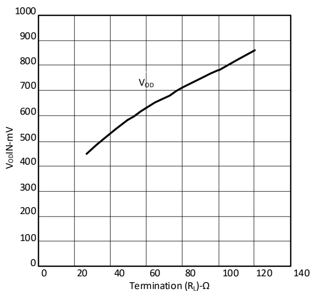
Figure 1. Typical V_{OD} Curve
