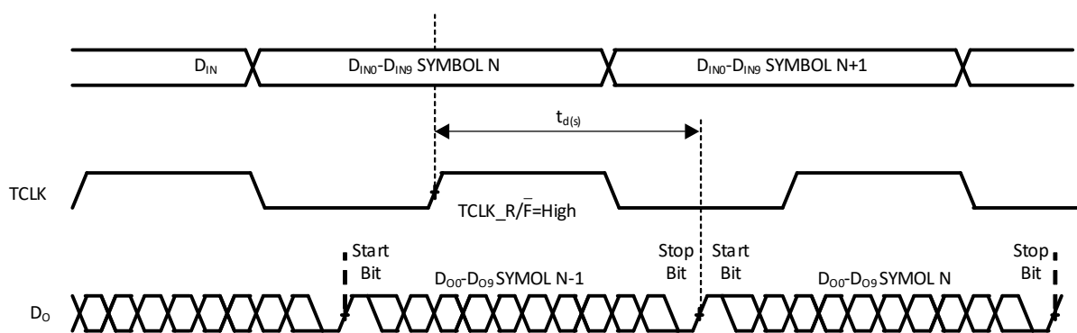
Figure 14. Serializer Delay
