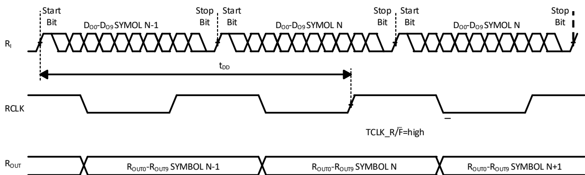
Figure 16. Deserializer Delay
