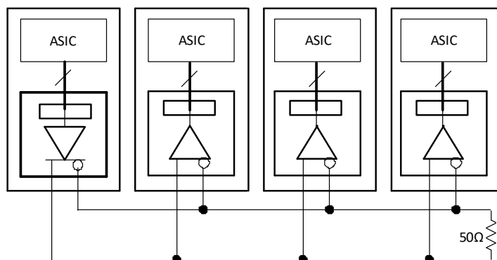
Figure 23. Multiconnection Configuration
