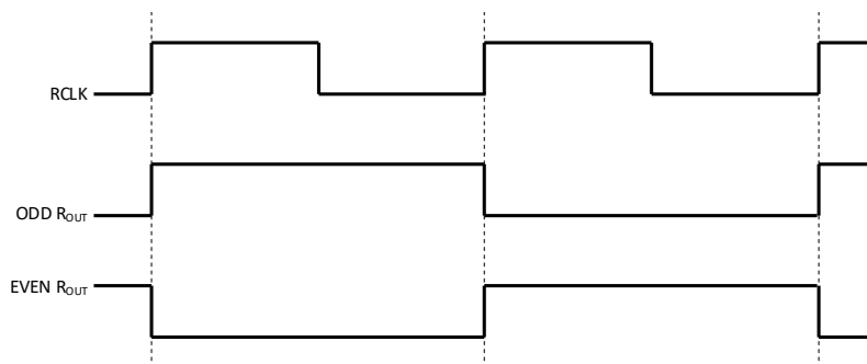
Figure 5. Worst-case Deserializer I_{CC} Test Mode
