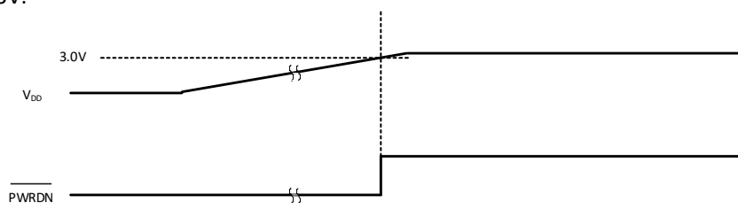
Figure 6. Device Start-up
