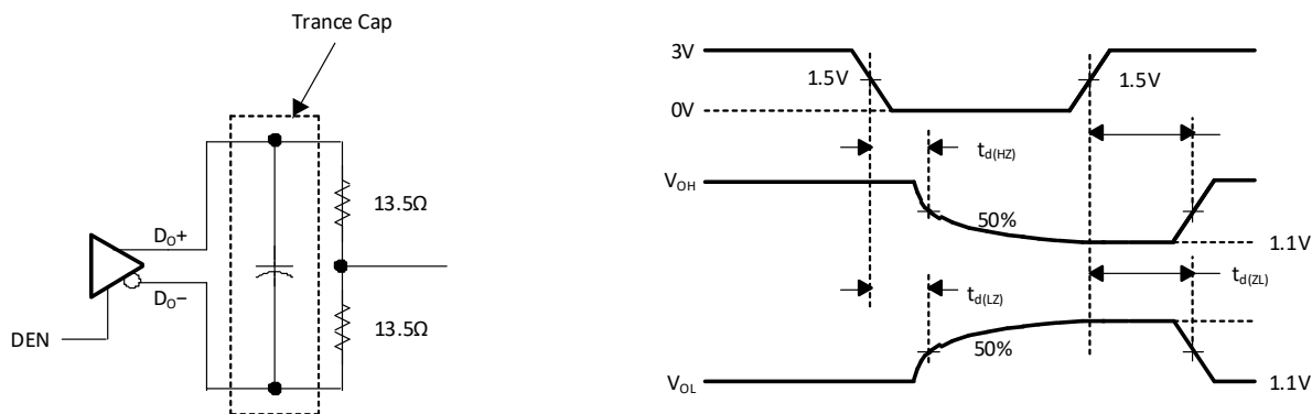
Figure 11. Serializer High-impedance-state Test Circuit and Timing
