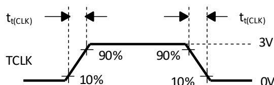
Figure 7. Serializer Input Clock Transition Time
