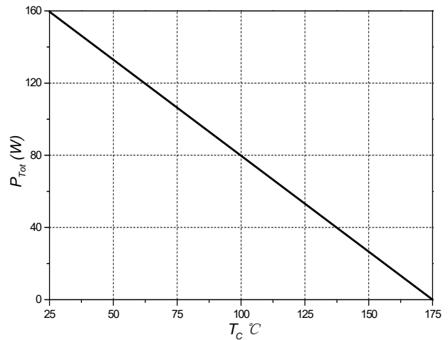
Figure 6. Power Derating
