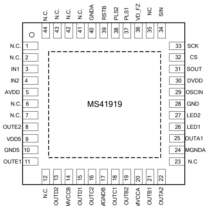
QFN44
