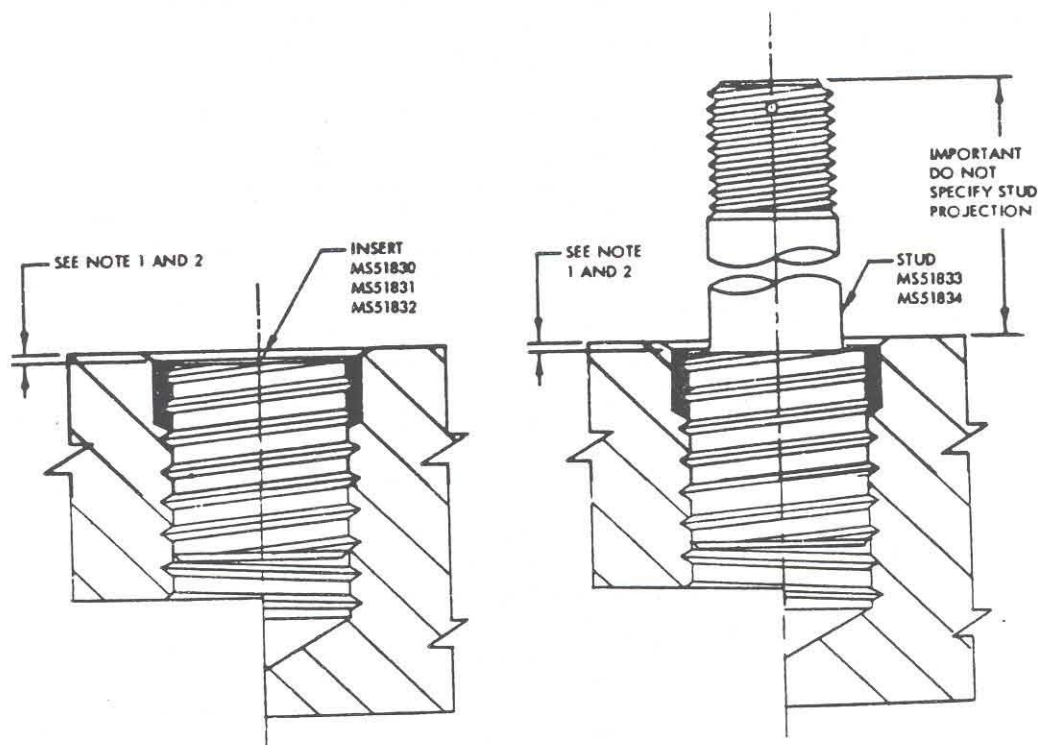
FIGURE II - ASSEMBLY OF INSERTS AND STUDS
