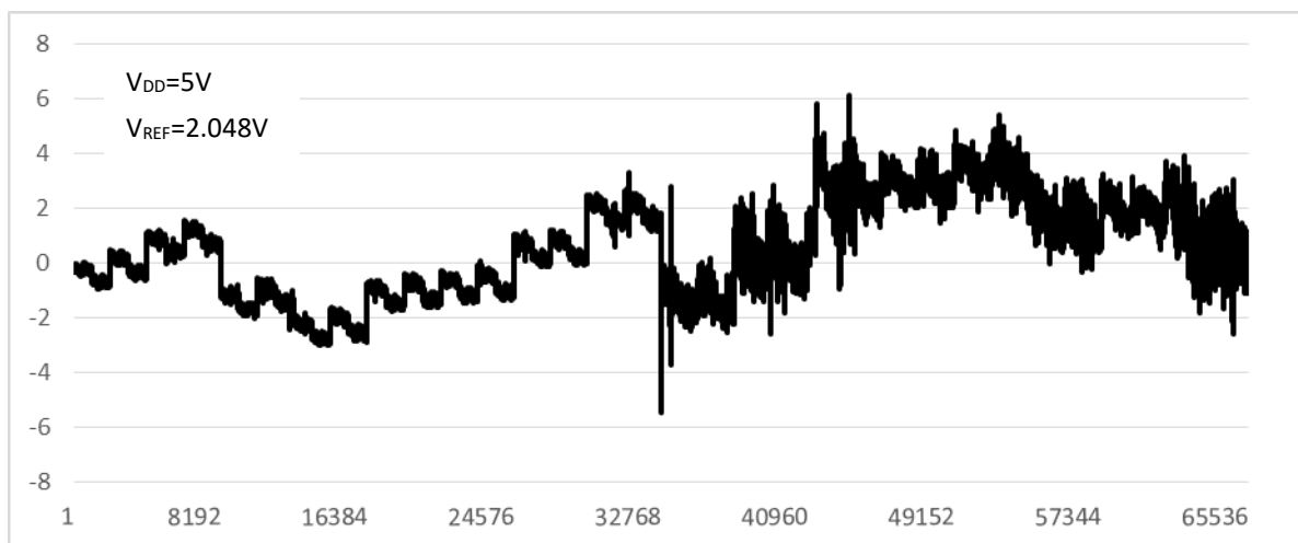
Figure 1. INL VS. Code
