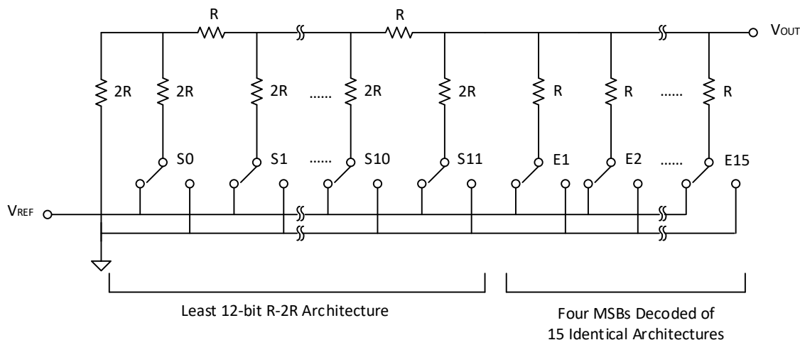
Figure 3. DAC Architecture
