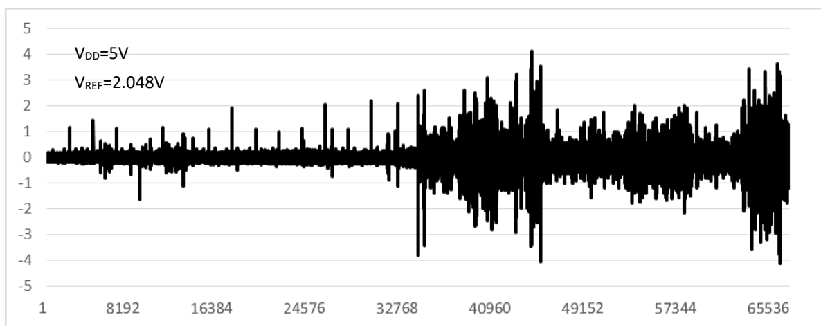
Figure 2. DNL VS. Code
