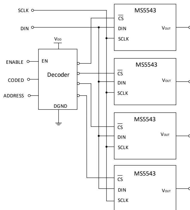
Figure 6. Multiple DACs
