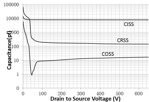
Capacitance Characteristics
