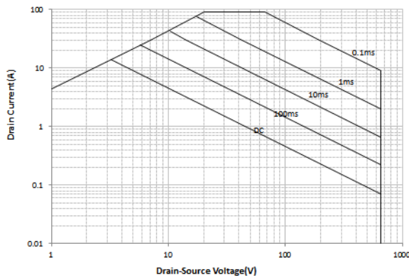
Maximum Safe Operating Area For MS65R120/TO-247
