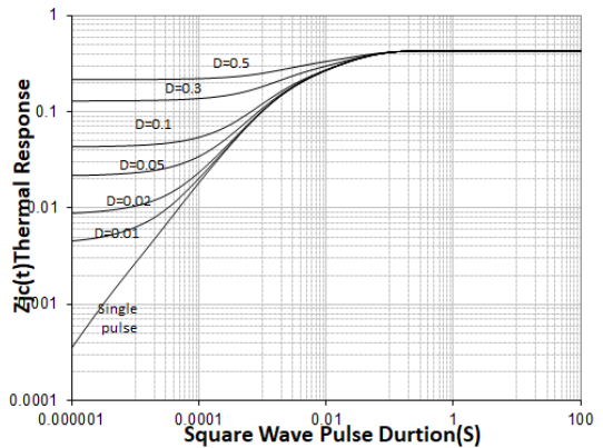
Transient Thermal Response Curve For MS65R120/TO-247
