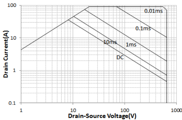
Maximum Safe Operating Area For MS65R120/TO-247
