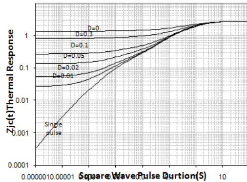
Transient Thermal Response Curve For MS65R120/TO-247
