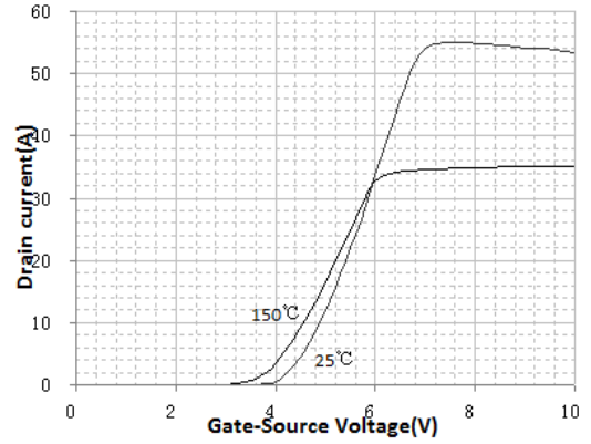
Transfer Characteristics
