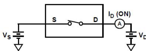
Leakage Current (On) Test Circuit
