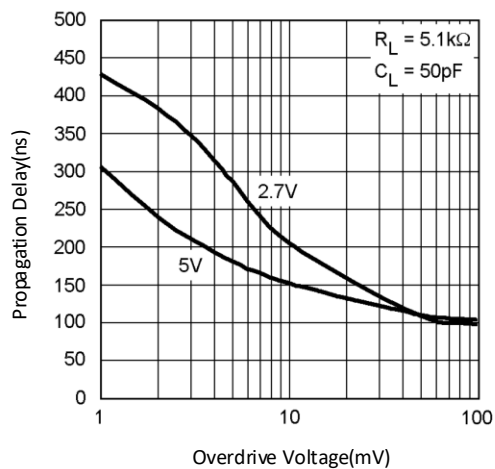
Propagation Delay VS. Overdrive Voltage
