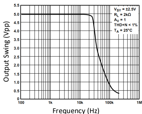
Maximum Output Swing VS. Frequency at 5V
