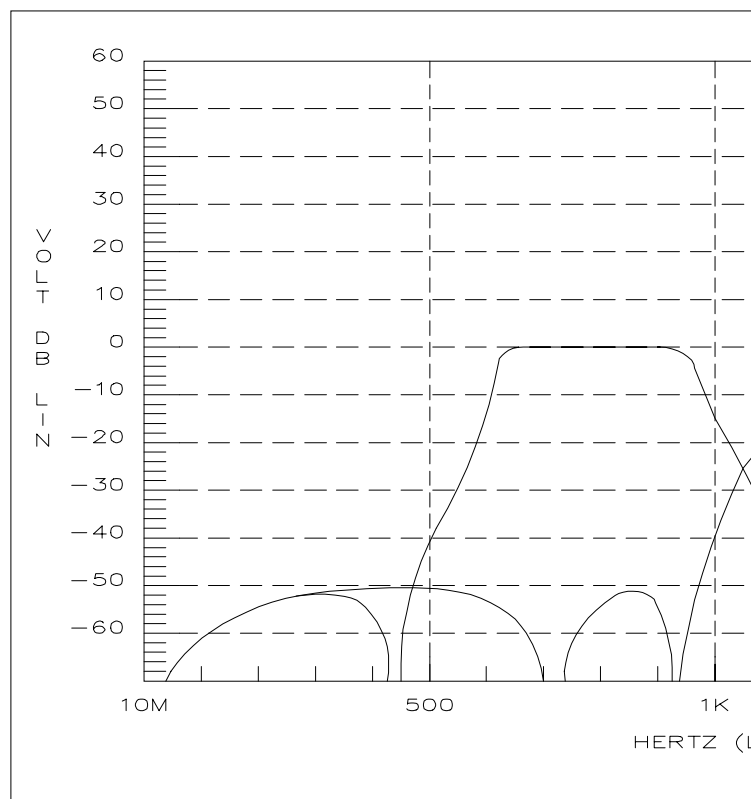
Figure 4. 6TH Order Bandpass
