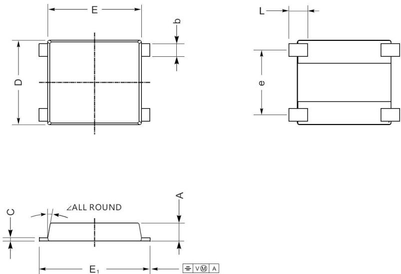
UMSB mechanical data
