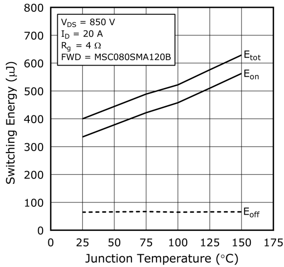
Figure 1-13. Switching Energy vs. Junction Temperature
