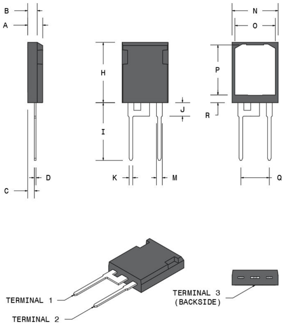
Figure 2-1. Package Outline Drawing
