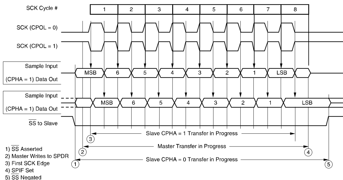
Figure 13-2. SPI Clock/Data timing
