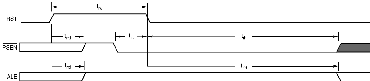
Figure 15-2. Serial Flash Programming Power-On Timing ( \overline{EA} is ignored)
