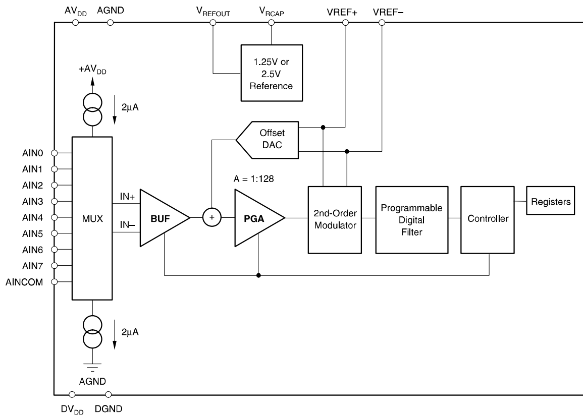
Figure 12-1. MSC1210 Architecture
