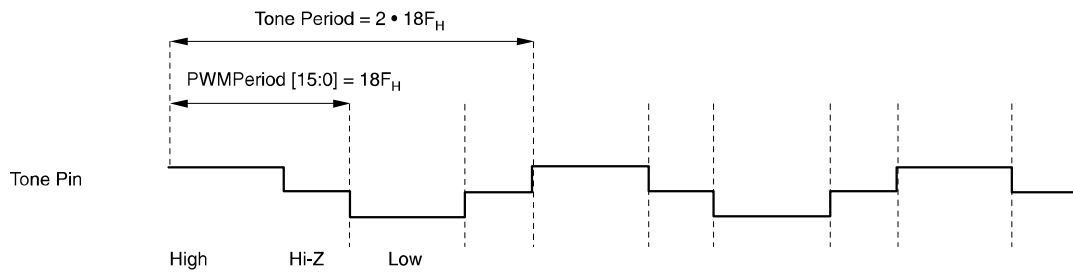
Figure 11-3. Timing Diagram of Tone Generator in Staircase Mode
