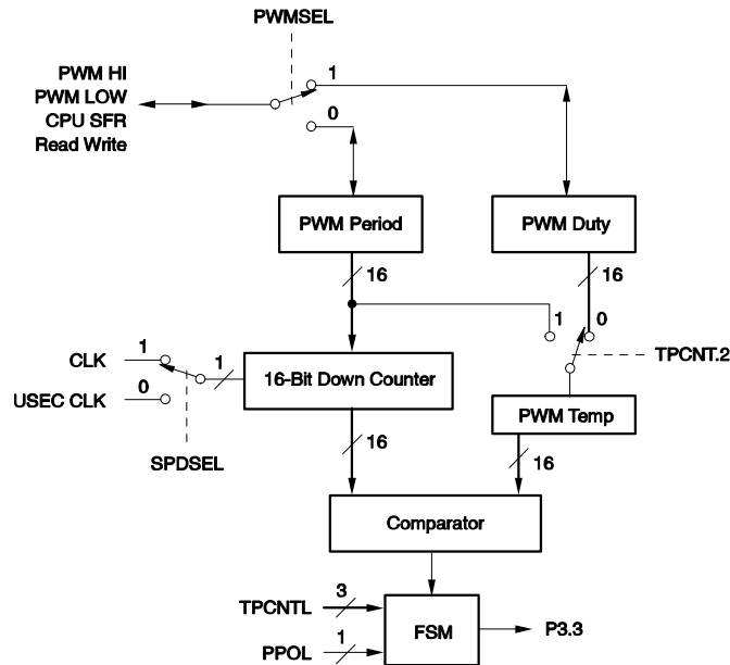
Figure 11-1. Block Diagram
