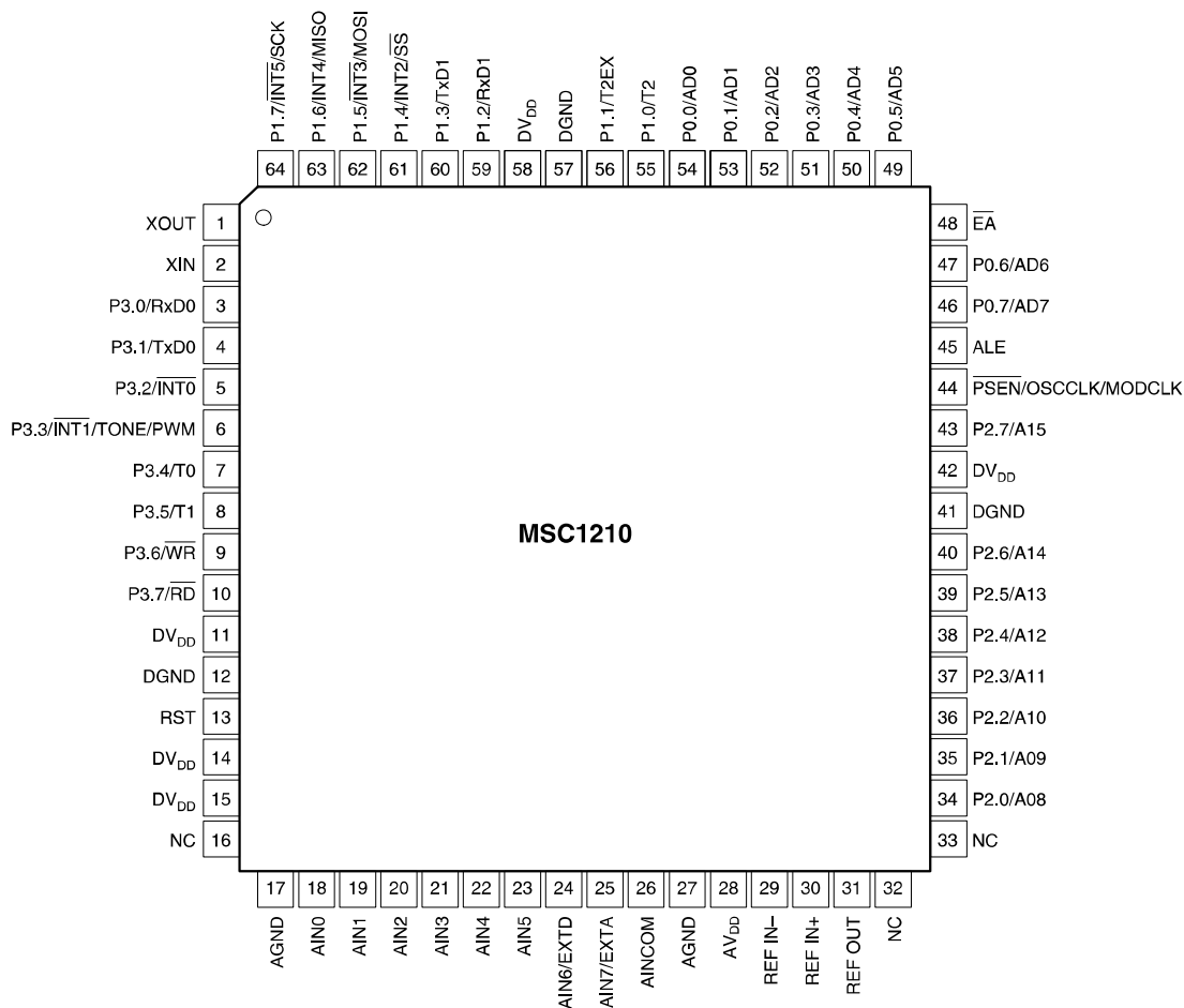
Figure 1-2. Pin Configuration of the MSC1210.
