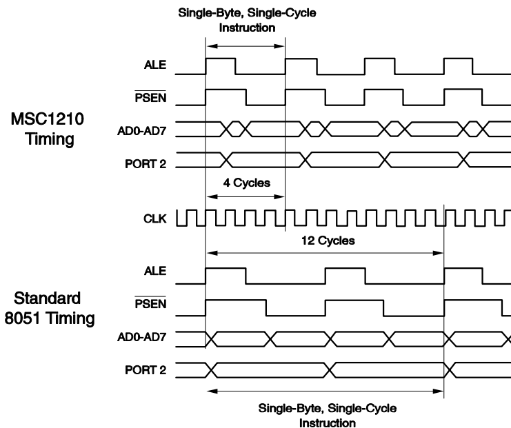
Figure 1-3. Timing Comparison of the MSC1210 to a Standard 8051.
