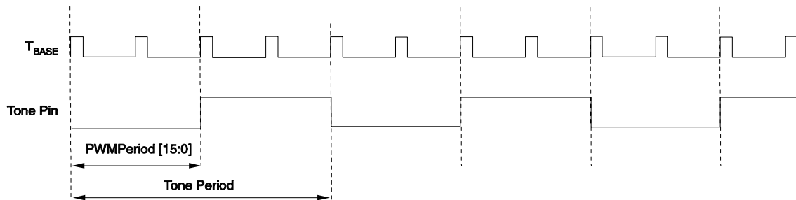
Figure 11-4. Timing Diagram of Tone Generator in Square Wave Mode
