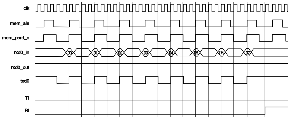
Figure 9-2. Serial Port Mode 0 Receive Timing—High Speed Operation.
