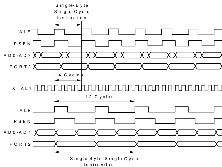
Figure 7-1. Standard 8051 Timing.
