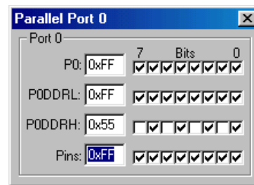
Figure 17-15. Parallel Port 0 Contents Display Window
