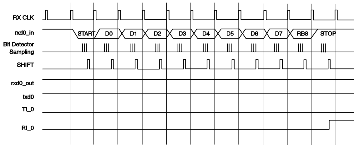
Figure 9-8. Serial Port 0 Mode 3 Receive Timing.
