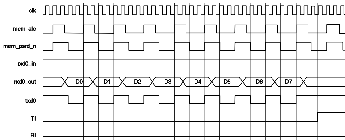
Figure 9-1. Serial Port 0 Mode 0 Transmit Timing—High Speed Operation.
