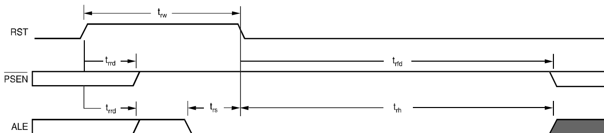
Figure 15-3. Parallel Flash Programming Power-On Timing ( \overline{EA} is ignored)
