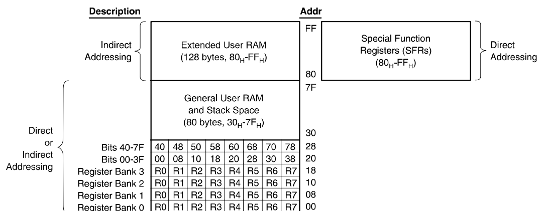
Figure 2-2. MSC1210 Memory Map Register Bank.
