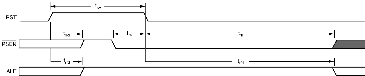
Figure 7-6. Serial Flash Programming Power-On Timing ( \overline{EA} is ignored)
