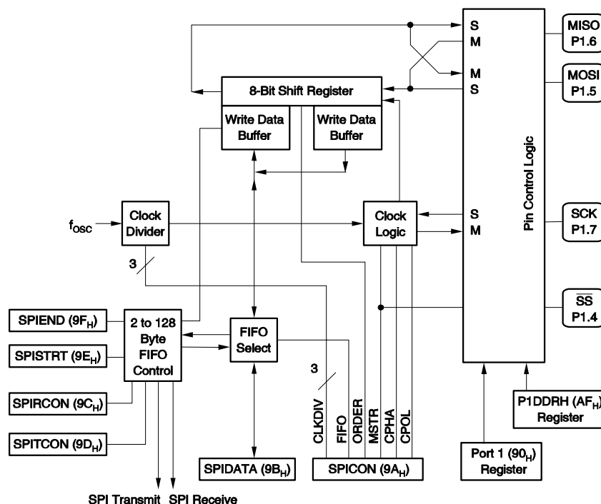
Figure 13-1. SPI block diagram
