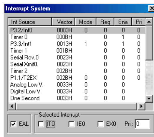
Figure 17-14. List Box for the Interrupt Peripheral
