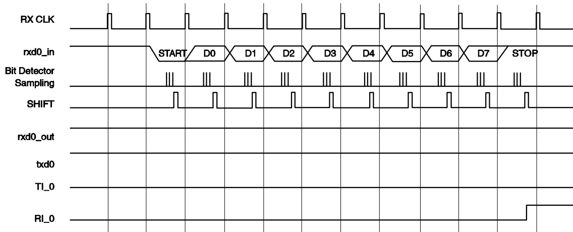
Figure 9-4. Serial Port 0 Mode 1 Receive Timing.
