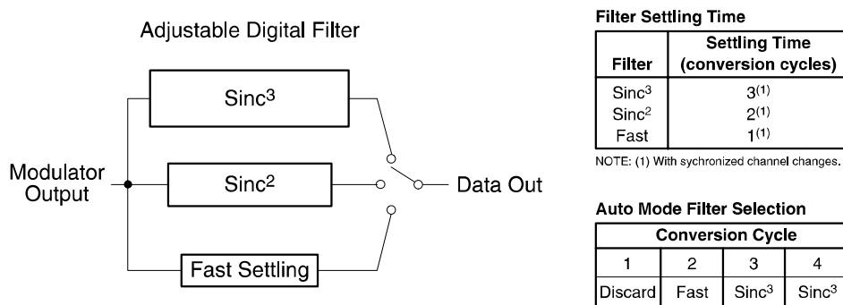
Figure 12-4. Filter Step Responses
