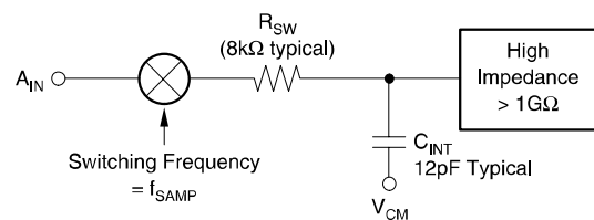
Figure 12-3. Basic Input Structure of the MSC1210
